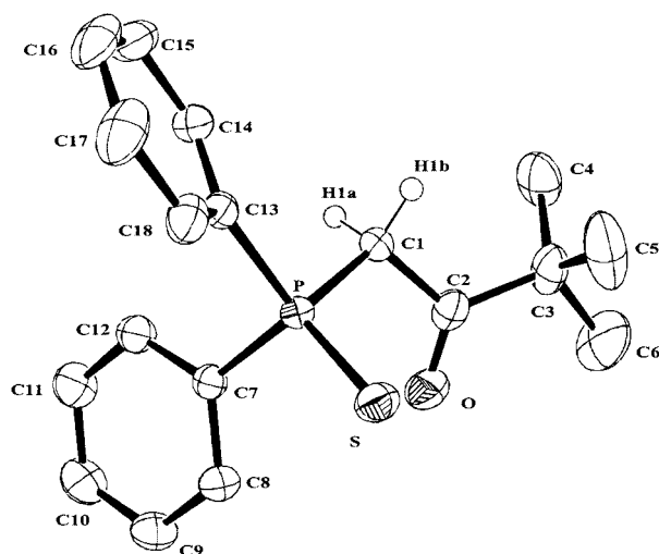
Figure 4. Molecular structure of \text{Ph}_2\text{P}(\text{S})\text{CH}_2\text{C}(\text{O})t\text{Bu} ( 9 ). Thermal ellipsoids are drawn at the 50% probability level. H atoms (except at C1) have been omitted for clarity.
