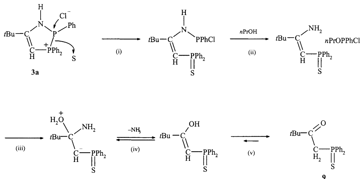
Scheme 3. Possible reaction mechanism for the formation of 9 .
