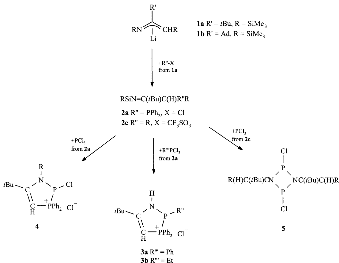
Scheme 1. Reactions of ketimines with phosphorus halides.
