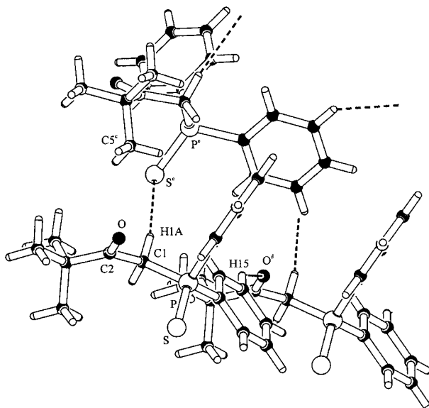
Figure 5. Intermolecular contacts in compound 9 . (For symmetry codes see Table 2).
