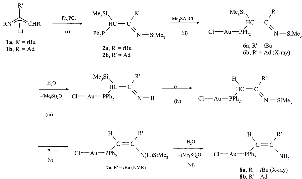
Scheme 2. Synthesis of gold phosphane complexes.
