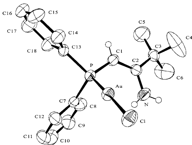
Figure 2. Molecular structure of ClAuPPh 2 CHC( t Bu)NH 2 ( 8a ). Thermal ellipsoids are drawn at the 50% probability level. H atoms (except at N, C1) have been omitted for clarity.
